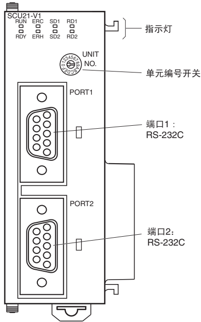
CJ1W-SCU21-V1/SCU22
