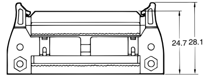
XG4T+XG4M+XG4E
