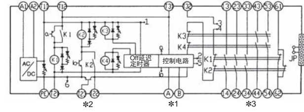
G9SA-TH301 (AC100V~240V)
