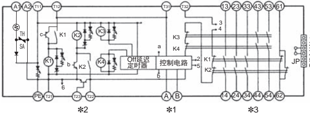
G9SA-TH301 (AC/DC24V)
