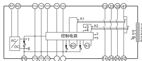
G9SA-TH301 (AC100V~240V)
